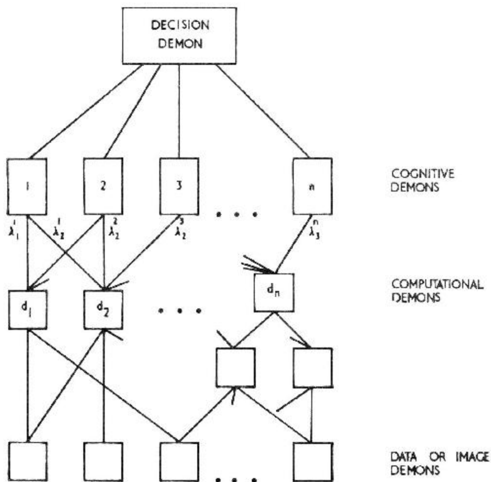
Fig. 3. Amended Pandemonium
